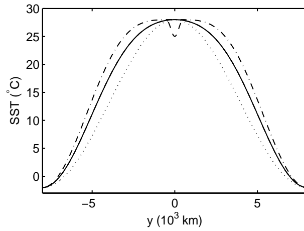
Figure 1: SST forcings for k = 0 (dotted), k = 0.6 (solid), and k=1 (dash-dotted); SST forcing for k=0.6 with a relative minimum at the equator (dashed).
