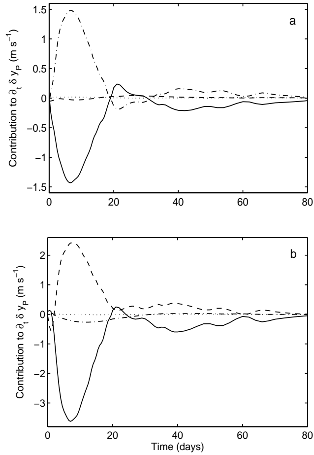
Figure 6: Contributions of the different processes to the return to the asymmetric equilibrium: (a) contributions of advection (solid), diffusion (dash-dotted), surface fluxes (dashed) and other terms (dotted) to \delta \dot{y}_p ; (b) contributions of barotropic vertical (solid) and horizontal (dotted) advections, baroclinic vertical (dashed) and horizontal (dash-dotted) advections.
