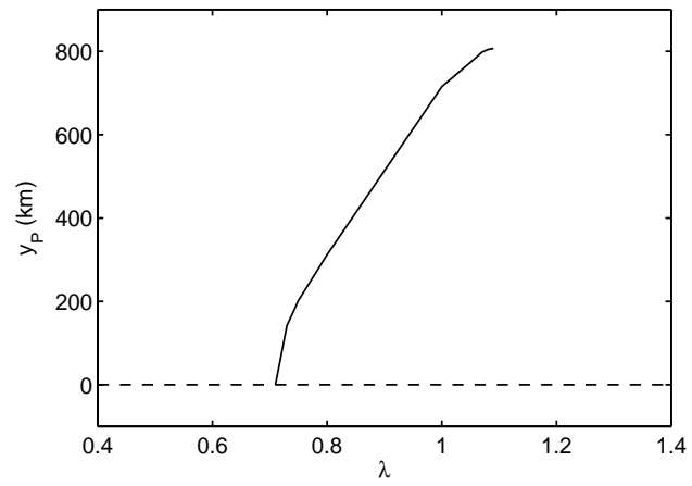
Figure 8: Latitude of the maximum of precipitation as a function of \lambda for the symmetric equilibrium (dashed) and the asymmetric equilibrium (solid).
