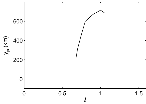
Figure 7: Latitude of the maximum of precipitation as a function of \ell for the symmetric equilibrium (dashed) and the asymmetric equilibrium (solid).
