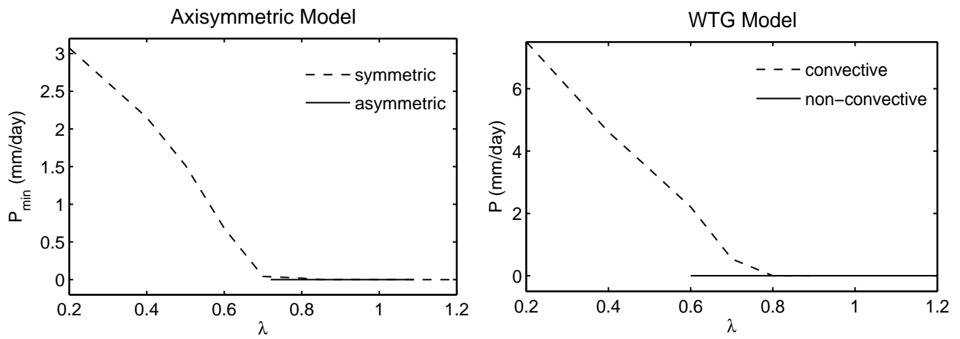
Figure 10: Subtropical precipitation minimum in the axisymmetric QTCM2 in the symmetric and asymmetric equilibria (left), and precipitation in the convective and non-convective equilibria of the WTG model (right) as a function of \lambda .
