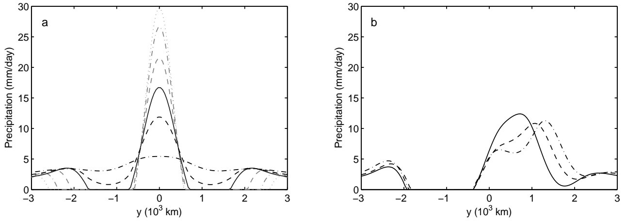
Figure 2: Precipitation for different symmetric SST forcings: (a) symmetric equilibrium for k = 0 (gray, dotted), k = 0.2 (gray, dash-dotted), k = 0.4 (gray, dashed), k = 0.6 (solid), k = 0.8 (dashed), and k = 1 (dash-dotted); (b) asymmetric equilibrium (with the ITCZ in the northern hemisphere) for k = 0.6 (solid), k = 0.8 (dashed), and k=1 (dash-dotted) .
