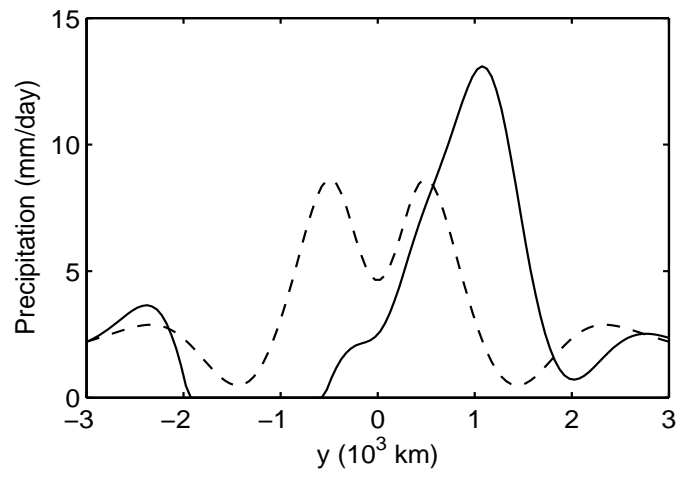
Figure 11: Precipitation in the symmetric (dashed) and asymmetric (solid) equilibria for a forcing with a relative minimum at the equator.
