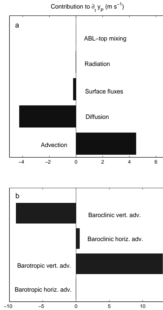
Figure 3: Contributions of the different processes to the position of the maximum of precipitation in the asymmetric equilibrium.
