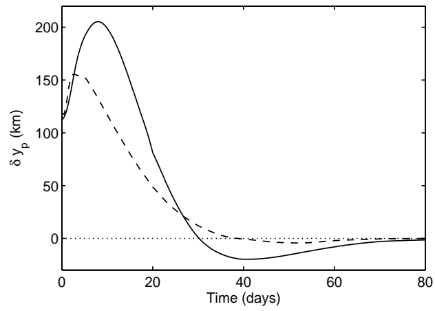
Figure 4: Time evolution of \delta y_p for the symmetric equilibrium (dashed) and the asymmetric equilibrium (solid).
