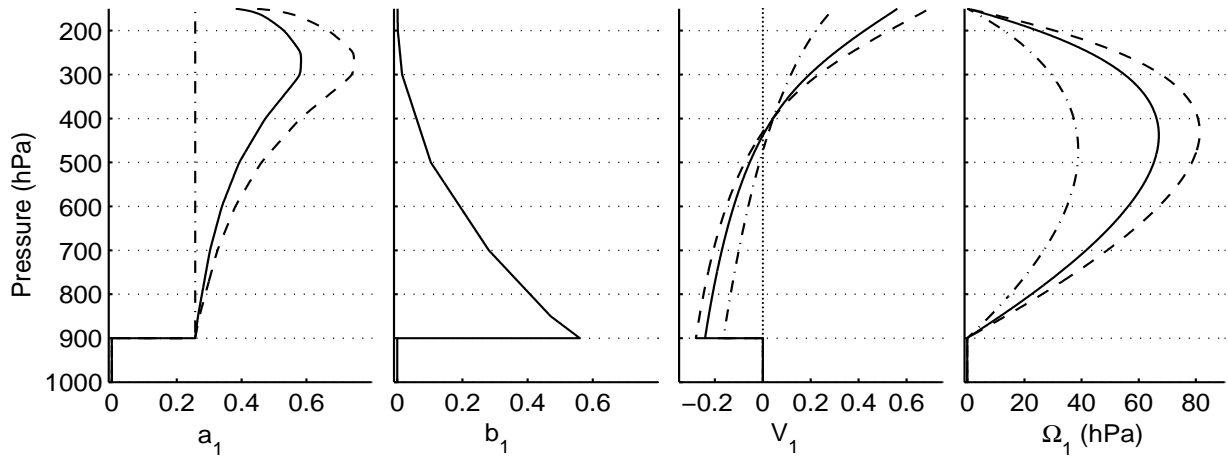
Figure 12: Free-tropospheric basis functions for temperature a_1 and humidity b_1 , horizontal wind V_1 , and vertical wind \Omega_1 (solid); a'_1 and the corresponding momentum functions V'_1 and \Omega'_1 are shown for \ell = 0 (dash-dotted), and for \ell = 1.5 (dashed).
