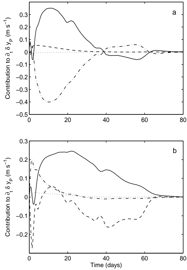
Figure 5: Contributions of the different processes to the return to the symmetric equilibrium: (a) contributions of avection (solid), diffusion (dash-dotted), surface fluxes (dashed) and other terms (dotted) to \dot{\delta y}_p ; (b) contributions of barotropic vertical (solid) and horizontal (dotted) advectons, baroclinic vertical (dashed) and horizontal (dash-dotted) advectons.
